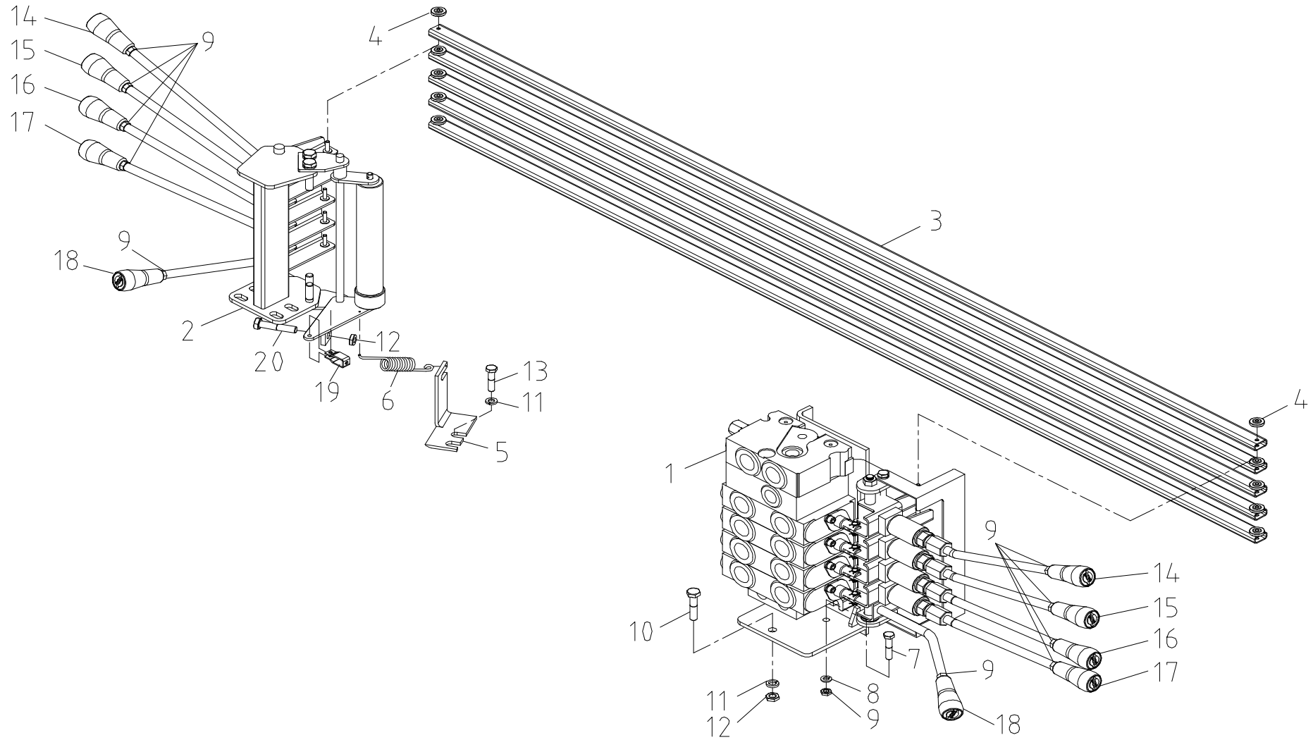
Fig. 3-5 SCS333 OPERATION MAIN ASS'Y(II)
