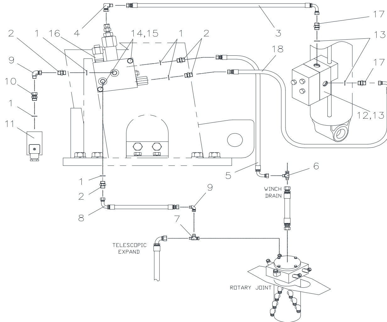
Fig. 5-7 SCS333 LOAD LIMMIT PIPING
