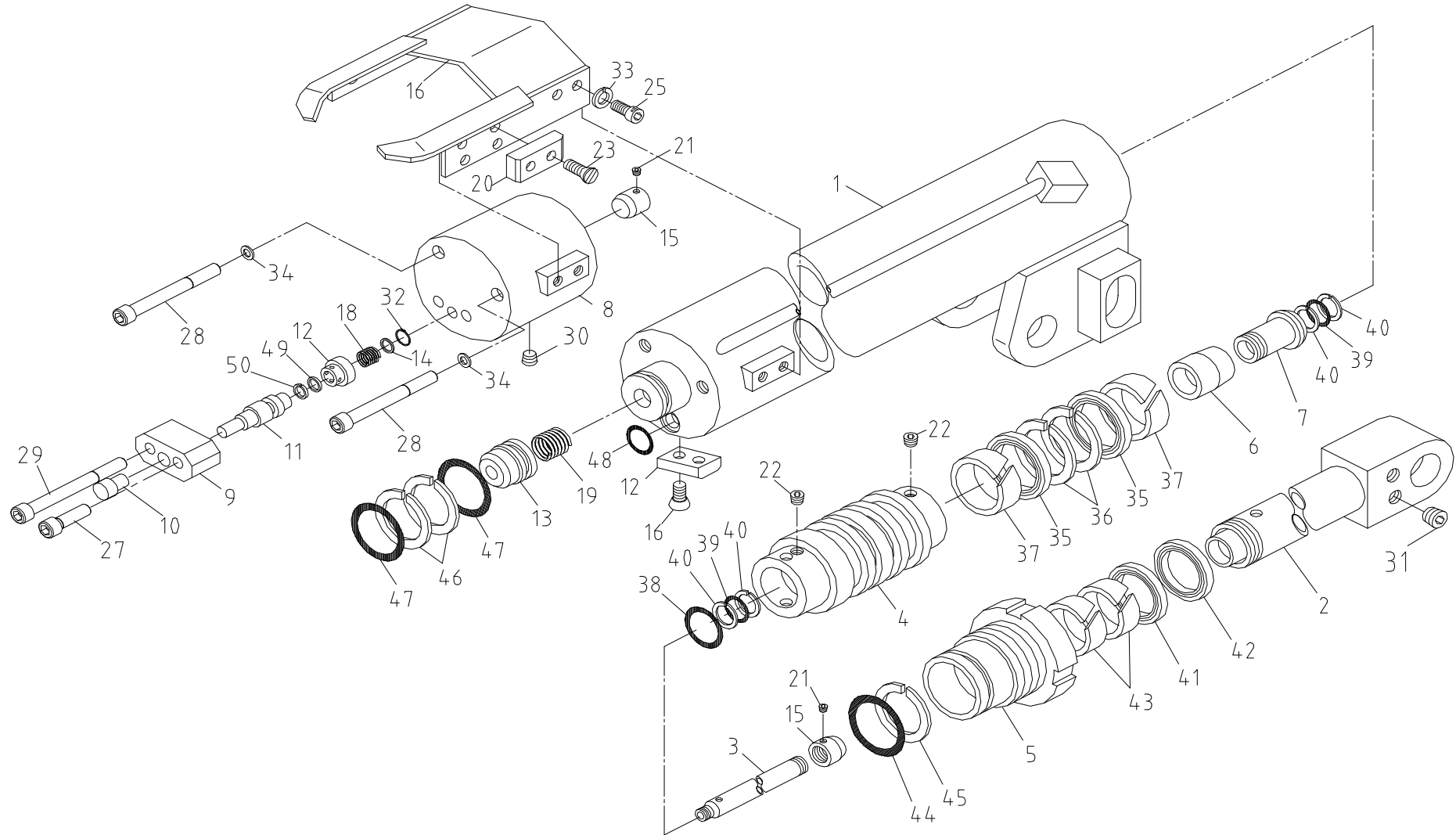
Fig. 1-1-1 SCS335 TELESCOPE CYL'(1st) ASS'Y
