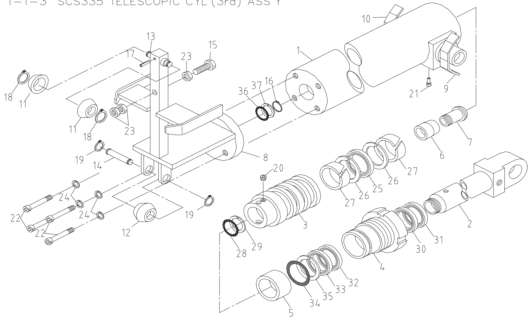
Fig. 1-1-3 SCS335 TELESCOPIC CYL'(3rd) ASS'Y
