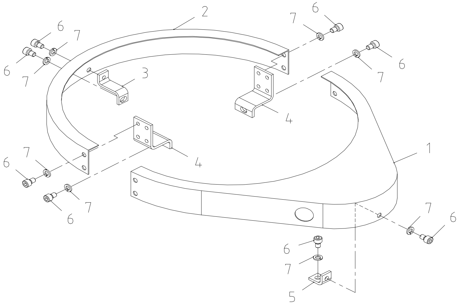
Fig. 3-3 SCS333 GEAR COVER ASS'Y
