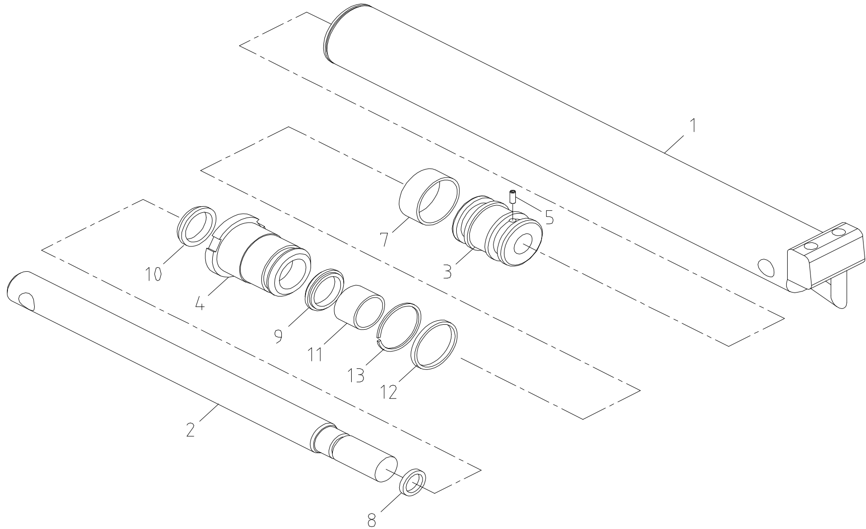
Fig. 4-2 SCS333 EXPAND CYL' ASS'Y
